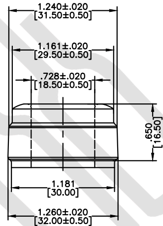
FINISH DETAIL SCALE 2:1
